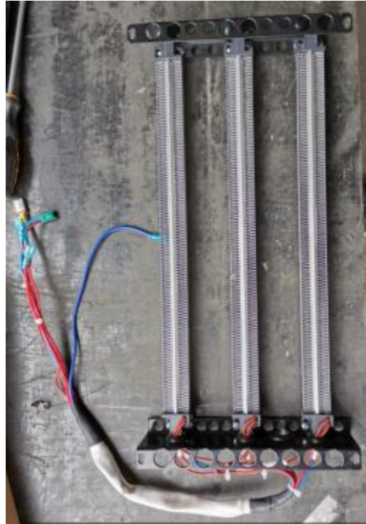
heating element
